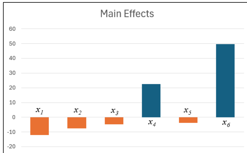
Figure 3 – DOE Main Effects Results
