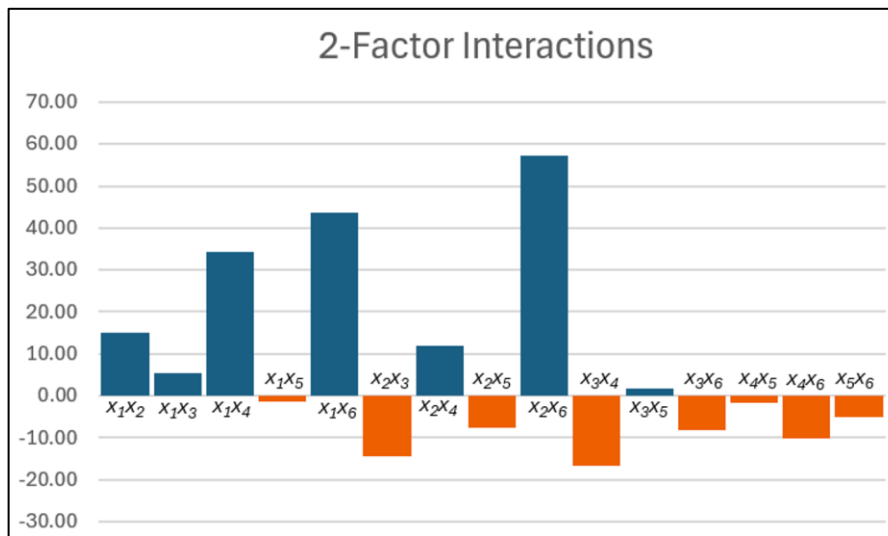
Figure 4 – DOE 2-Factor Interactions Results
